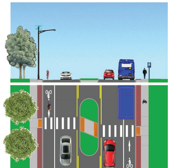
Delaware Avenue 3 Lane Concept
